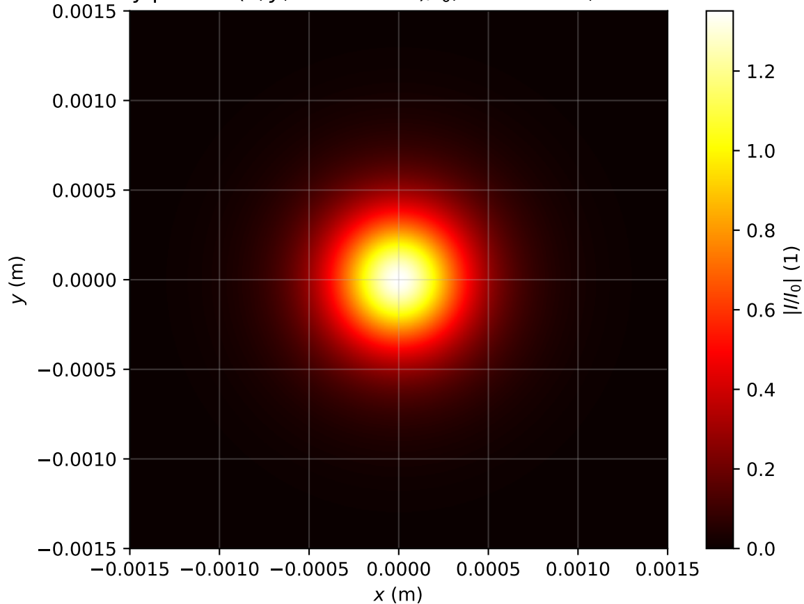
Intensity profile I(x, y, z = 1.353m)/I_0 , \text{Pin}=0.8\text{Pcr} , artificial time
